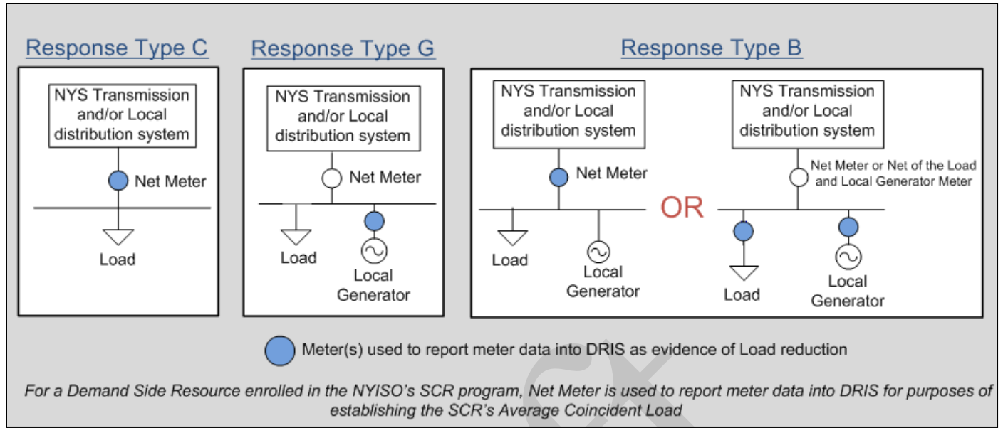
Figure 5-1 Examples of acceptable Meter Configurations
